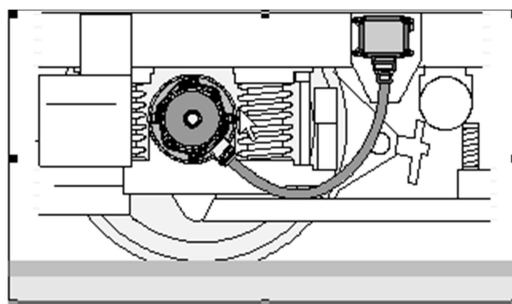
Figure 31: Wheel Sensor
